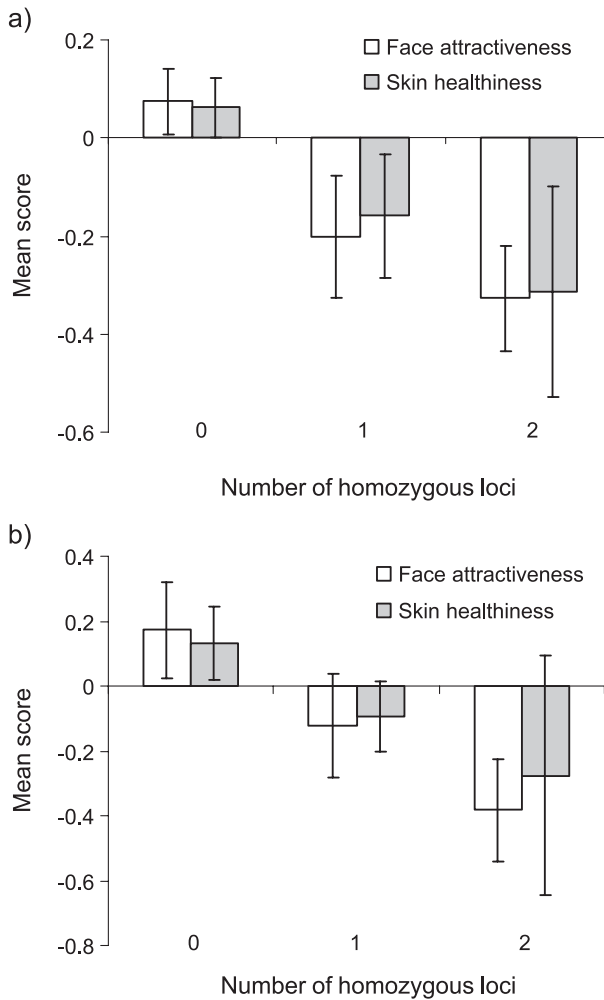
Fig. 1. Facial attractiveness and skin healthiness ratings of men with different numbers of homozygous MHC loci. (a) Ratings are means ( \pm S.E.) of standardised scores given by 50 women (Study 1). Sixty-nine men were heterozygous at all three loci, 19 were homozygous at one locus, and 4 were homozygous at two loci. (b) Ratings from 36 genotyped women (Study 2); n = 56 men heterozygous at all three loci, 16 men homozygous at one locus, and 4 homozygous at two loci.
