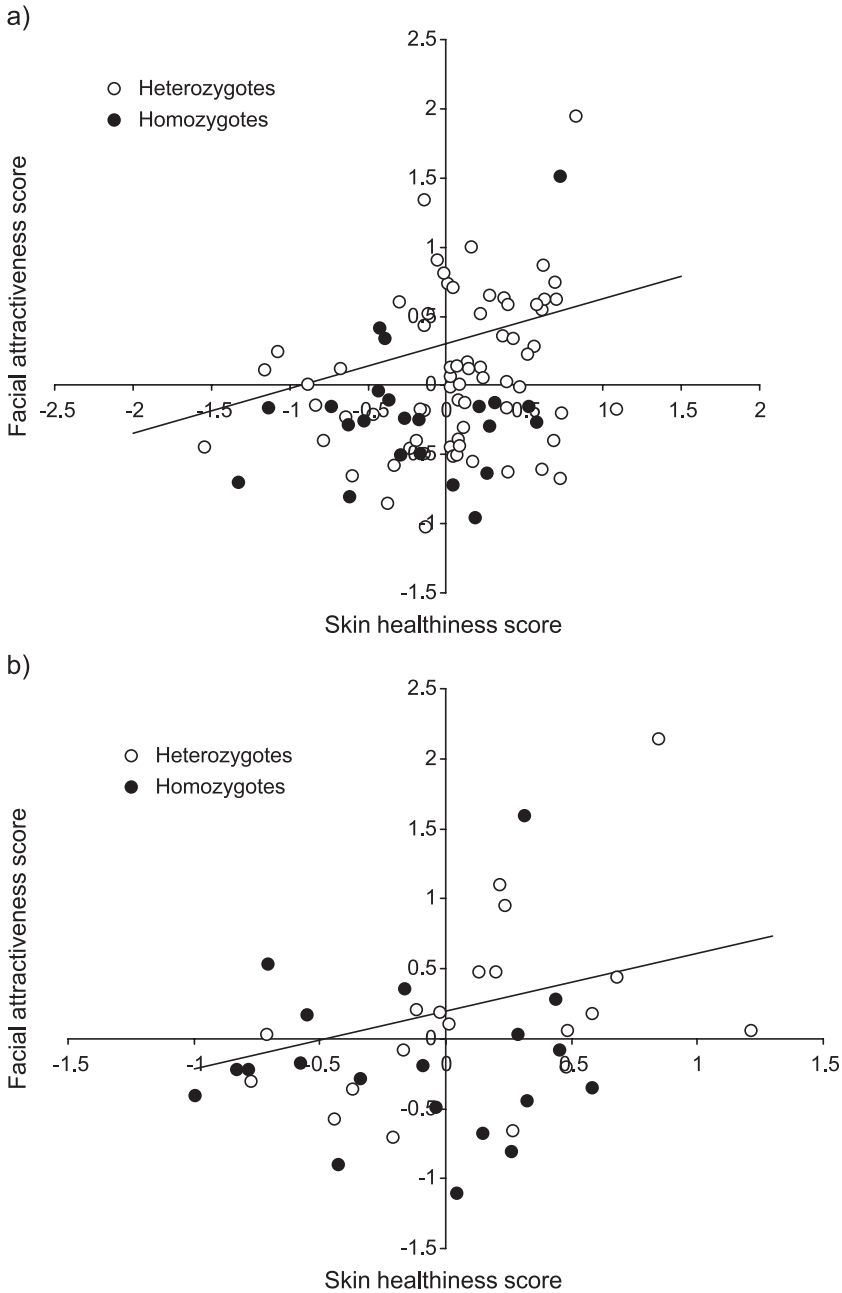
Fig. 2. Correlation between facial attractiveness and skin healthiness scores. (a) Mean scores for 92 men rated in random order by 50 women, with scores for each variable standardised within rater to control for differential use of the scale (Study 1). (b) Mean scores of 20 heterozygotes and 20 homozygotes, randomly selected from the 92 men, rated by a second group of 36 genotyped women (Study 2). Mean ratings of whole-face attractiveness for each man were positively correlated with mean skin healthiness ratings (a: p = .004 ; b: p = 0.041 ).
